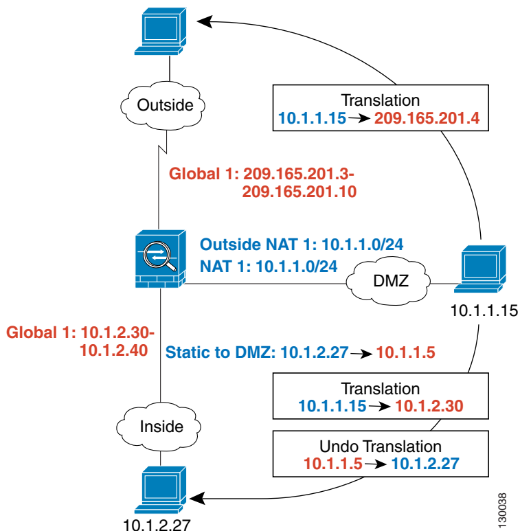
Figure 19-20 Outside NAT and Inside NAT Combined
