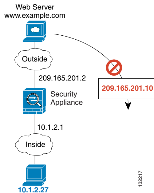
Figure 19-7 Remote Host Attempts to Initiate a Connection to a Mapped Address
